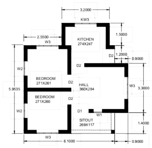
GROUND FLOOR PLAN AREA :43.7M 2 (470SQFT)
